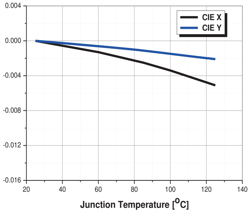
Fig 8. Junction Temp. vs. CIE X, Y Shift, I_F=640\text{mA}
