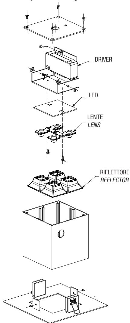
LED Equal 4 R montaggio ad incasso LED Equal 4 R ceiling mount
