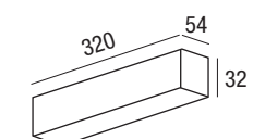
Rosone per Driver (driver escluso) Driver box (driver not included)
