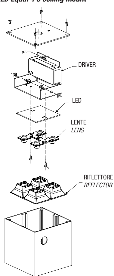
LED Equal 4 C montaggio a soffitto LED Equal 4 C ceiling mount
