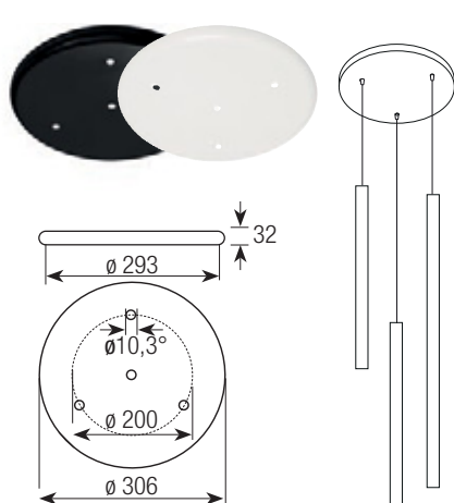
ROSONE TONDO Ø 305 - 4 FORI ROUND CEILING ROSE Ø 305 - 4 HOLES
