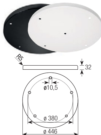
ROSONE TONDO Ø 445 - 5 FORI ROUND CEILING ROSE Ø 445 - 5 HOLES
