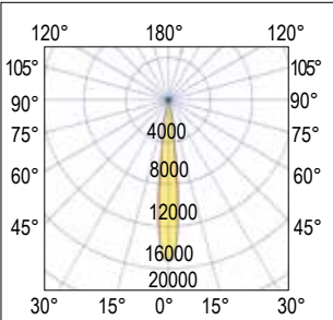
15° - Super spot
