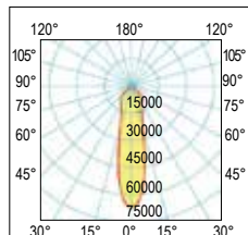
25° Semi-concentrate Semi-concentrating
