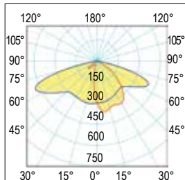
ST/CDL1 Ottica stradale consigliata per strade con pista ciclabile Road optics recommended for roads with cycle tracks
