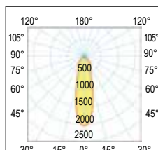
25° Semi-concentrante - Spot
